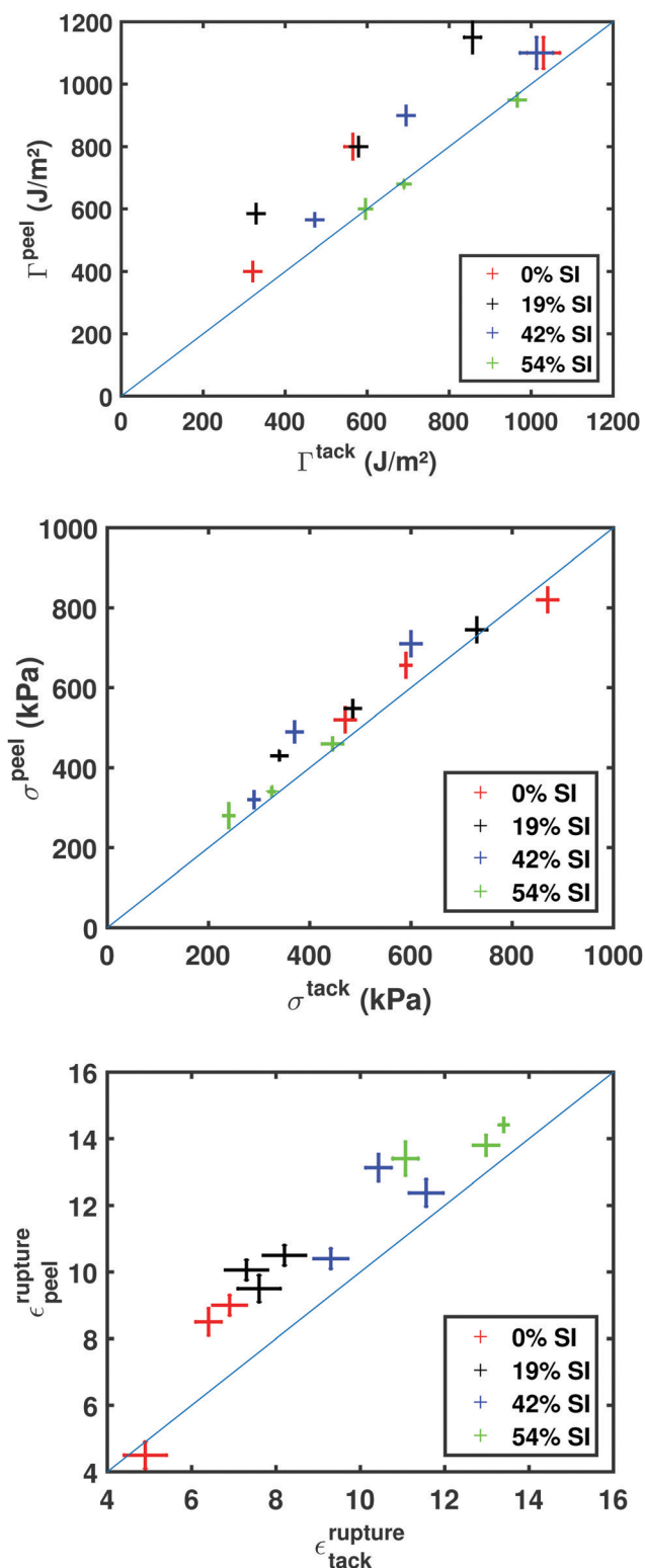
Fig. 10 Comparison of the adhesion energy, average stress and maximum fibril extension during peel and tack tests at the same fibril strain rate. The vertical and horizontal error bars represent the total scatter in the peel data and tack data, respectively.
