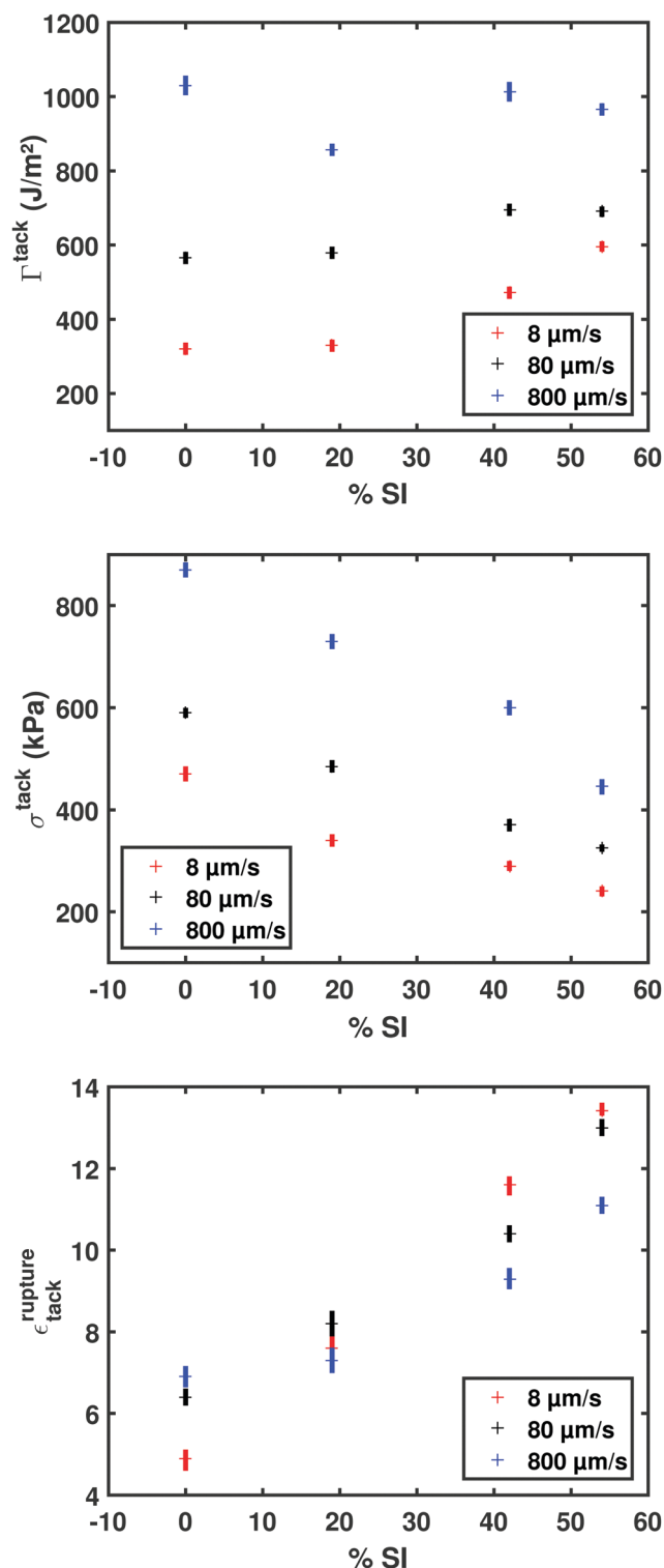
Fig. 9 Fracture energy, average plateau stress and maximum fibril strain derived from the tack curves as a function of the diblock content and peeling velocity. The vertical error bars represent the total scatter in the data.
