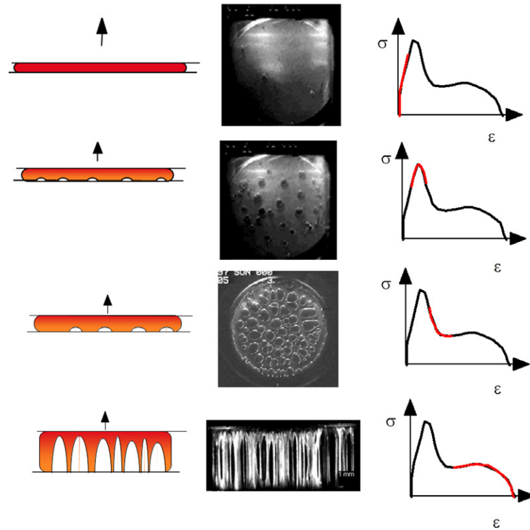
Figure 12. Schematic of the debonding mechanism of a soft adhesive from a rigid surface in a probe tack test. Reproduced with permission from Lakrouit et al (1999; copyright 1999 Taylor & Francis).
