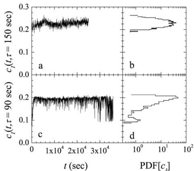
Fig. 3 For a representative ROI, degree of correlation c_I at a fixed delay \tau as a function of time and its PDF for the “artificial skin” in humid (RH = 62%, \tau = 150 s, panels a and b) and dry (RH = 12%, \tau = 90 s, panels c and d) atmosphere. Note that the dry sample exhibits large temporal fluctuations.
